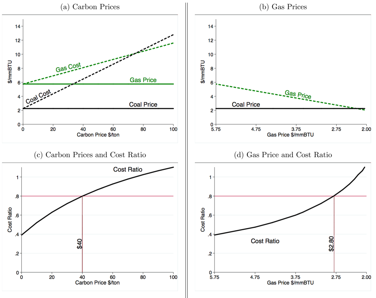
Figure 5: Relationship between Gas Prices, Carbon Prices, and Cost Ratios
